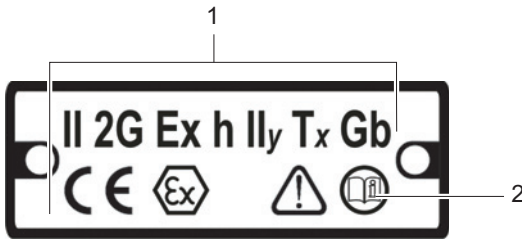
Fig. 2 Plaque ATEX (exemple)
